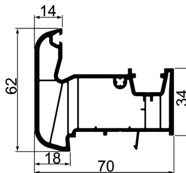
80/6 Promena smer
