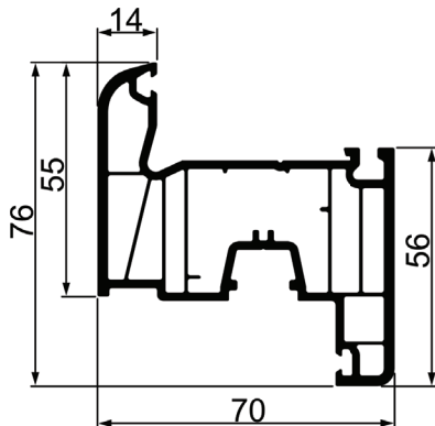
56/6 Krilo
